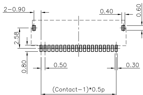
RECOMMENDED LAYOUT ( TOP VIEW) GENERAL TOLERANCE: ±0.05mm
