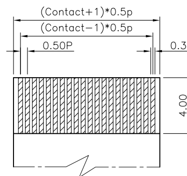
FFC/ FPC DIMENSION THICKNESS 0.3mm
