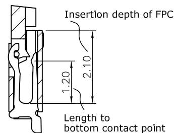
SECTION VIEW SCALE 10/1
