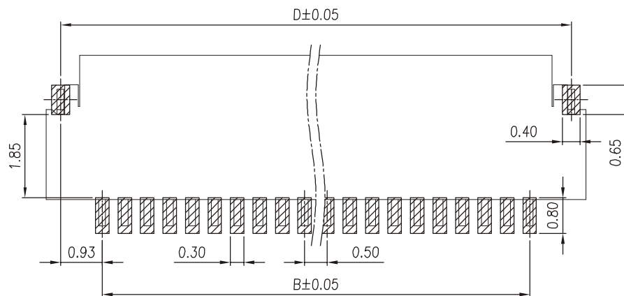
RECOMMENDED PCB LAYOUT Tolerance: \pm 0.05
