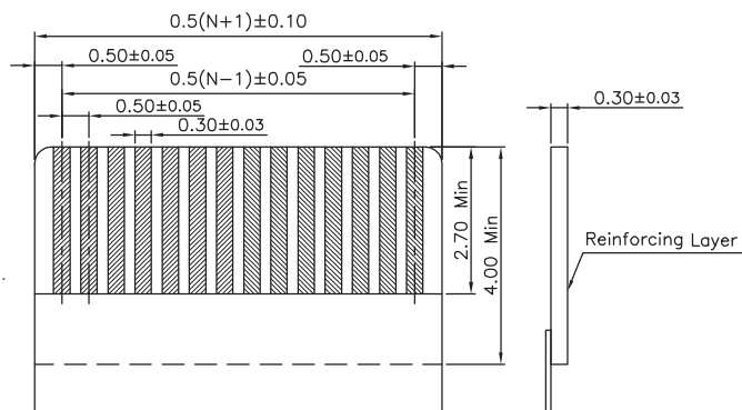
RECOMMENDED FFC/FPC DIMENSION
