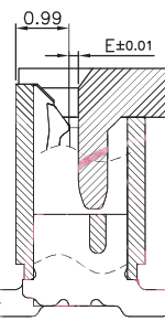
SECTION B-B
