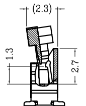
SECTION A-A Without cover
