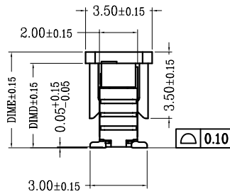
SECTION A-A Without cover
