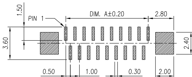
RECOMMENDED PCB LAYOUT TOLERANCE: \pm 0.05
