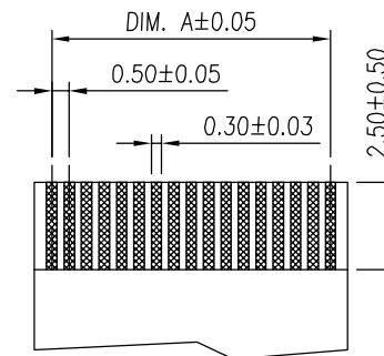
FFC/FPC DIMENSION THICKNESS 0.30 \pm 0.03 mm
