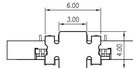
CAP PLACEMENT DIAGRAM
