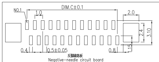
Negative-needle circuit board
