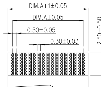
FFC/FPC DIMENSION THICKNESS 0.30±0.03 mm
