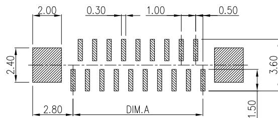
RECOMMENDED P.C.B. LAYOUT TOLERANCE: ±0.05
