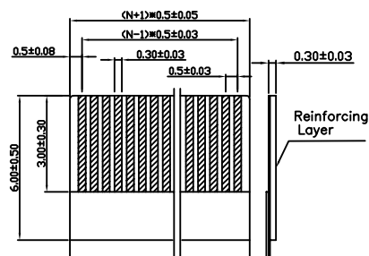
RECOMMENDED FFC/FPC DIM.
