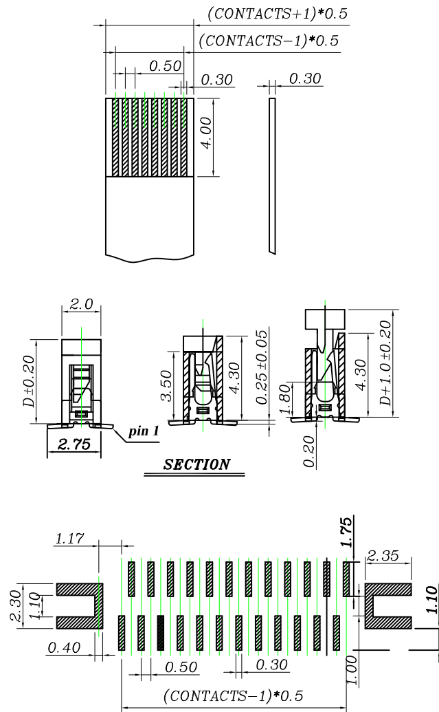
PC BOARD LAYOUT
