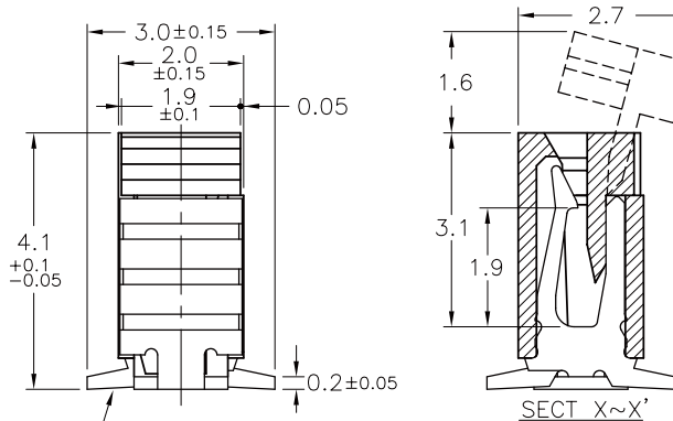
NO.1 Contact
