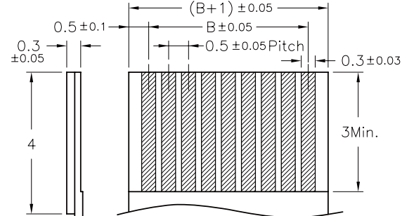
Applicable FPC
