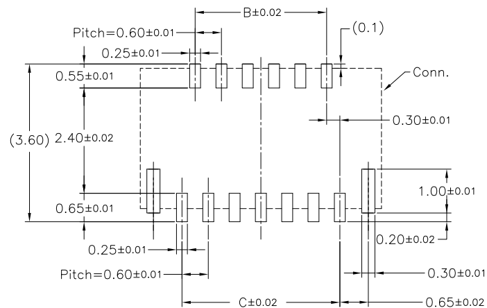
RECOMMENDED METAL MASK PATTERN(THICKNESS 0.1mm)
