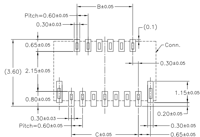
RECOMMENDED METAL MASK PATTERN(THICKNESS 0.1mm)
