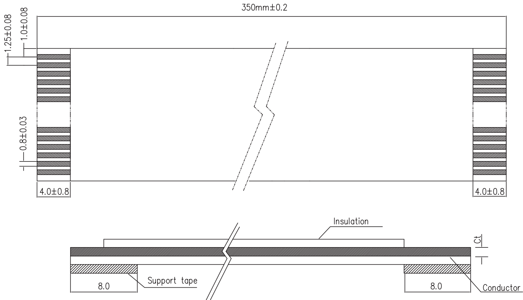
FFC 17 WAY FLAT FLEXIBLE CABLE UL20624 80°C 60V
