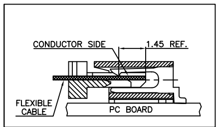
UPPER CONTACT
