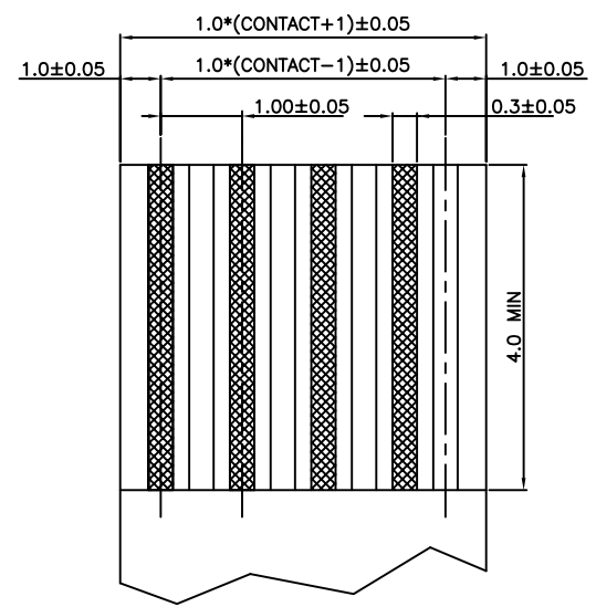
FFC/FPC DIMENSION THICKNESS 0.3 +0.03 -0.03 mm
