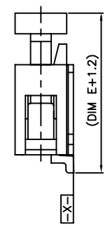
OPEN TYPE
