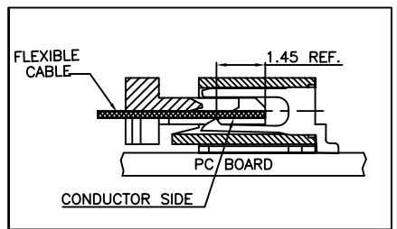
LOWER CONTACT
