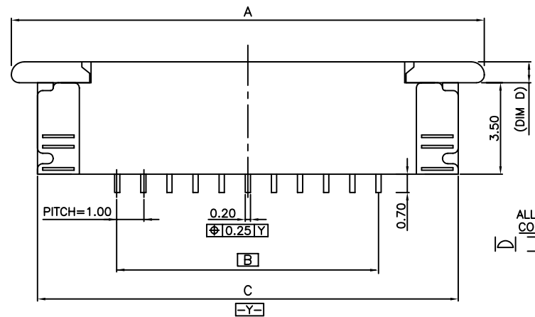
LOWER CONTACT
