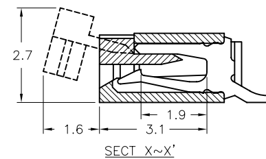
SECT. X~X'
