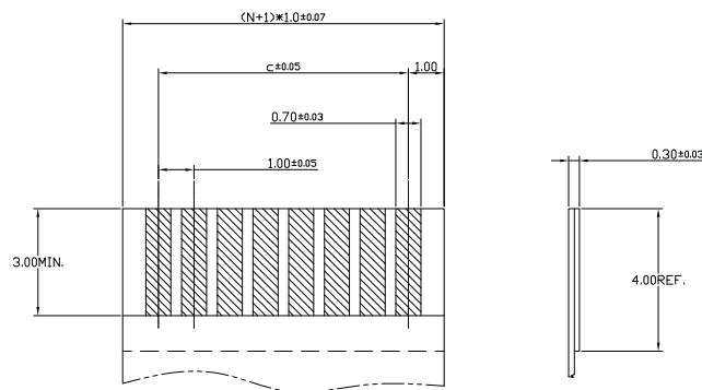
APPLICABLE FFC TOLERANCE:±0.05
