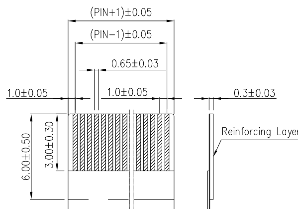
RECOMMENDED FFC/FPC DIM.
