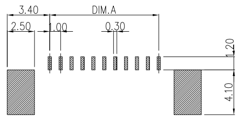
RECOMMENDED PCB LAYOUT TOLERANCE: ±0.05
