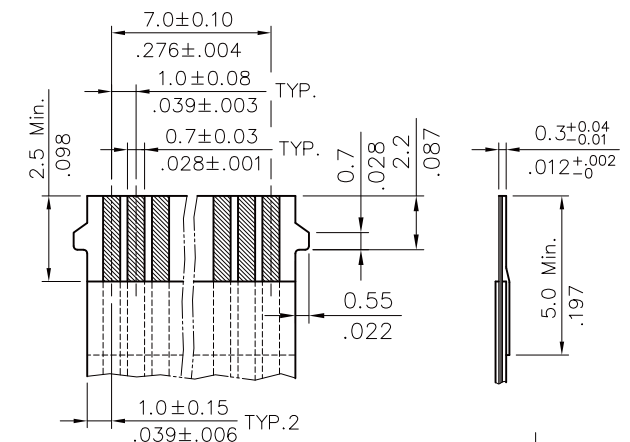
Accommodated FFC/FPC
