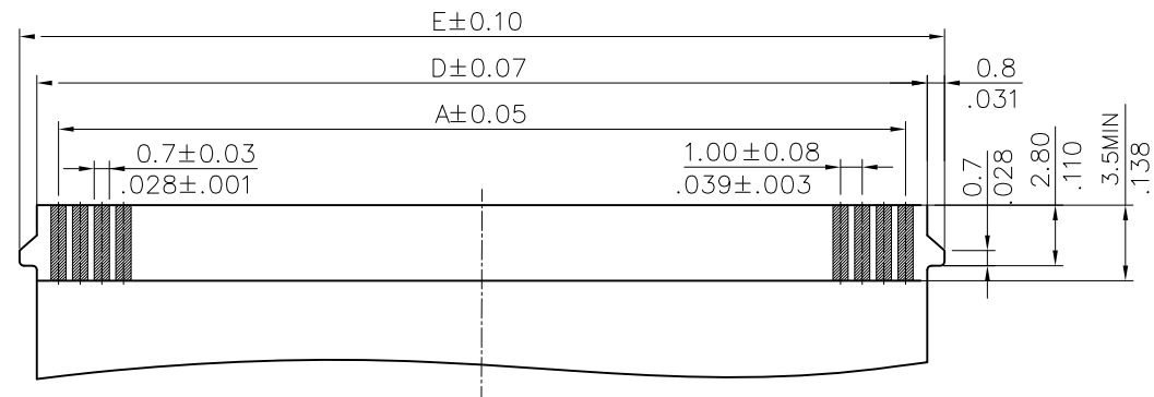
Accommodated FFC/FPC(TYPE1)
