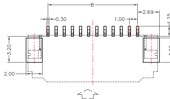
FPC/FFC Insert Direction
