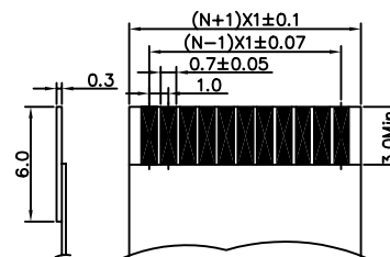
N=NUMBER OF CONTACTS (APPLICABLE FPC/FFC)
