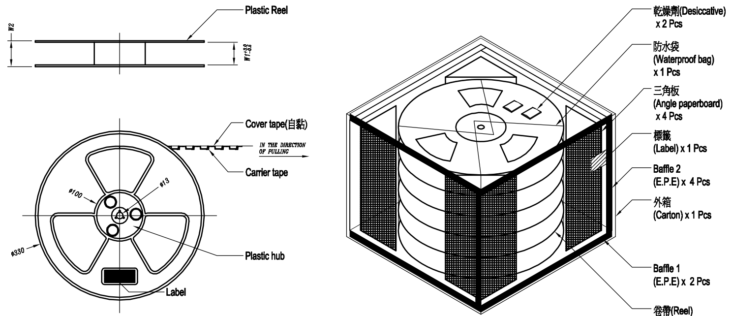
包裝示意圖(PACKAGING SCHEMATIC)
