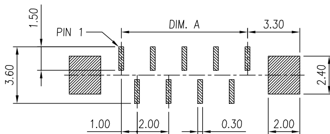
RECOMMENDED PCB LAYOUT TOLERANCE: \pm 0.05
