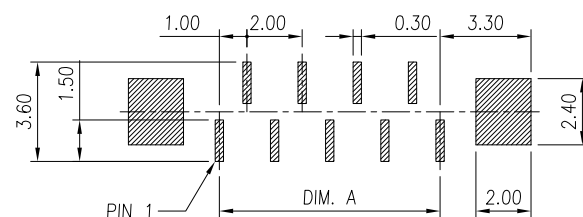
RECOMMENDED PCB LAYOUT TOLERANCE: ±0.05
