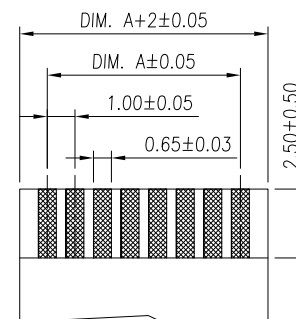
FFC/FPC DIMENSION THICKNESS 0.30 \pm 0.03 mm
