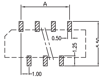
Negative Type PCB Layout
