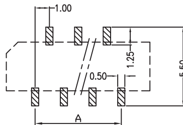
Positive Type PCB Layout
