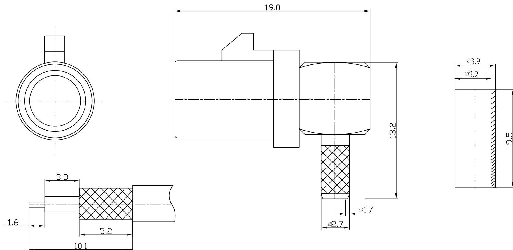
RECOMMENDED STRIPPING DIMENSIONS
