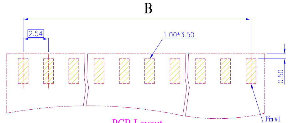
PCB Layout (Both Sides)
