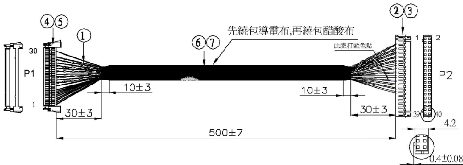
P1 WIRE COLOR P2 1 RED 19 2 RED 20 3 RED 21 4 RED 22 5 BLACK 13 6 BROWN 14 7 ORANGE 15 8 YELLOW 16 9 GREEN 28 10 NC 11 BLUE 17 12 BLACK TWIST PAIR 10 13 WHITE 9 14 PURPLE 18 15 BROWN TWIST PAIR 8 16 WHITE 7 17 GRAY 23 18 RED TWIST PAIR 6 19 WHITE 5 20 WHITE 24 21 ORANGE TWIST PAIR 12 22 WHITE 11 23 BLACK 25 24 YELLOW TWIST PAIR 4 25 WHITE 3 26 BROWN 26 27 NC 28 NC 29 ORANGE 27 30 NC
