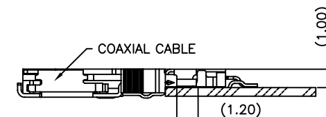
MATED CONDITION(REF)
