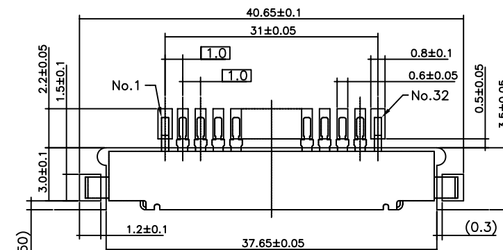
APPLICABLE PCB DIMENSION(REF)
