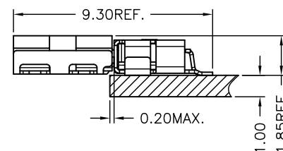
MATED CONDITION
