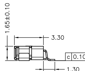
MATED CONDITION
