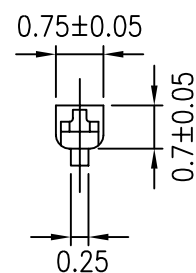
B-B SECTION
