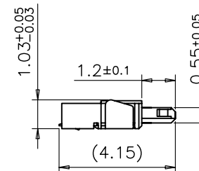
With Lock
