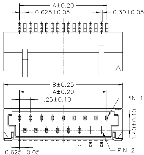
13,15,17,19,21,31,41 Contacts
