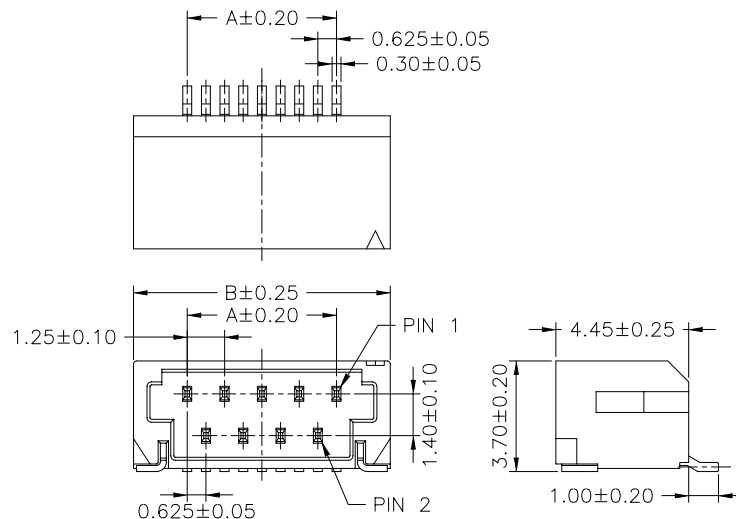
5,7,9,11 Contacts
