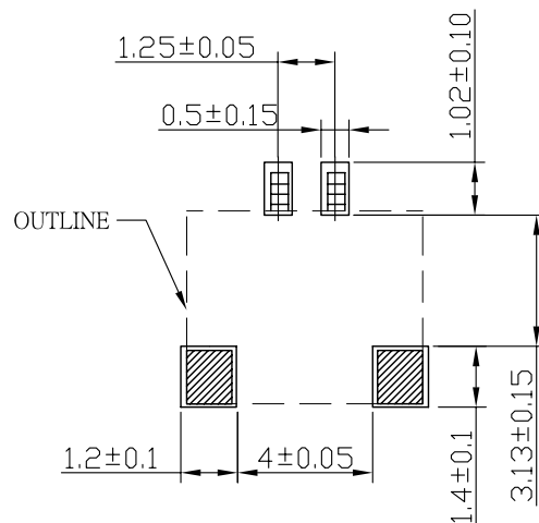
RECOMMENDED P.C. BOARD PATTERN DIM.
