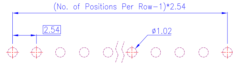
PCB Layout (Top View)
