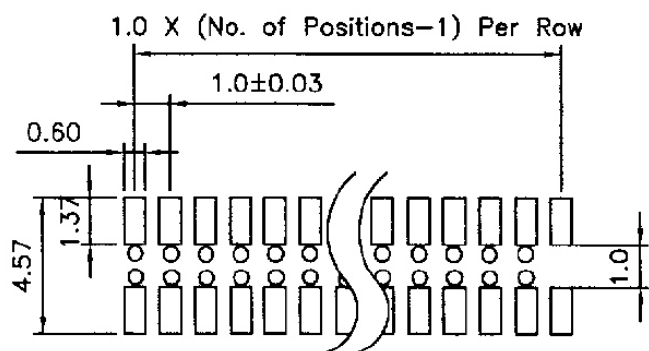
RECOMMENDED P.C.B LAYOUT (TOP VIEW) TOLERANCES: ±0.05mm
