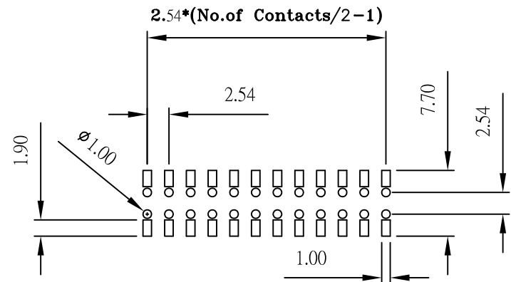
Recommended P.C. Board SMD Layout
