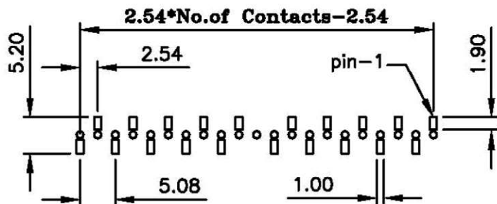
Recommended P.C. Board SMD Layout
