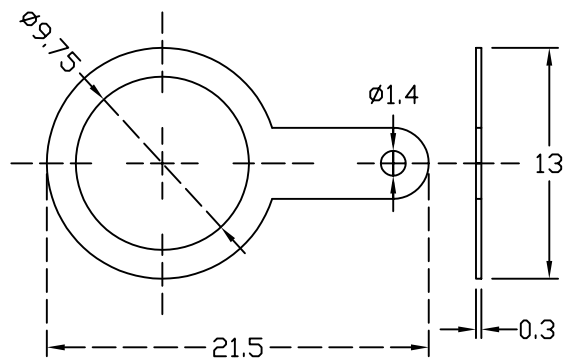
( SOLDER TAG )
