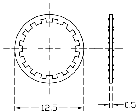
( LOCK WASHER )
