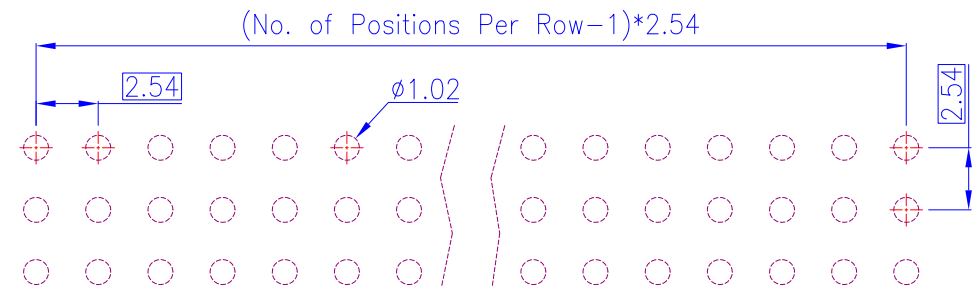
PCB Layout (Top View)
