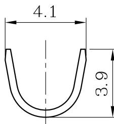
SEC. B-B
