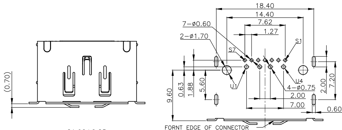
REFERENCE PC BOARD LAYOUT TOP VIEW (TOL=±0.05)
