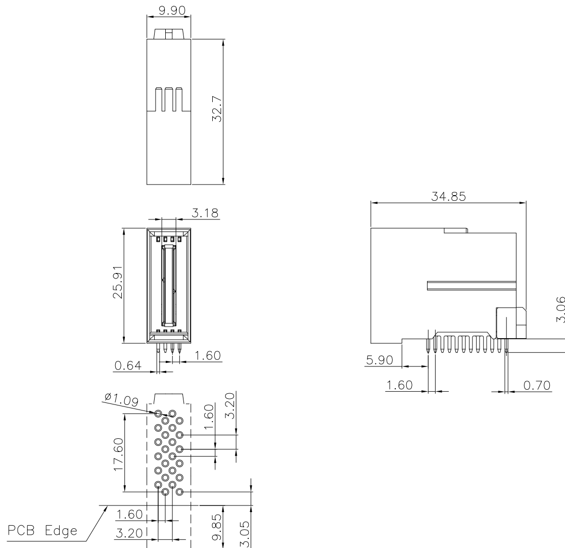
P.C. Board Layout (Tolerance:±0.05)
