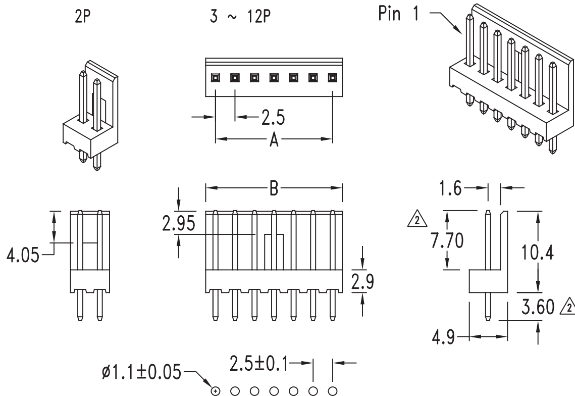
P. C. board hole dimensions
