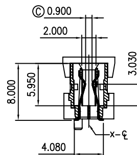
SEC. A-A'
