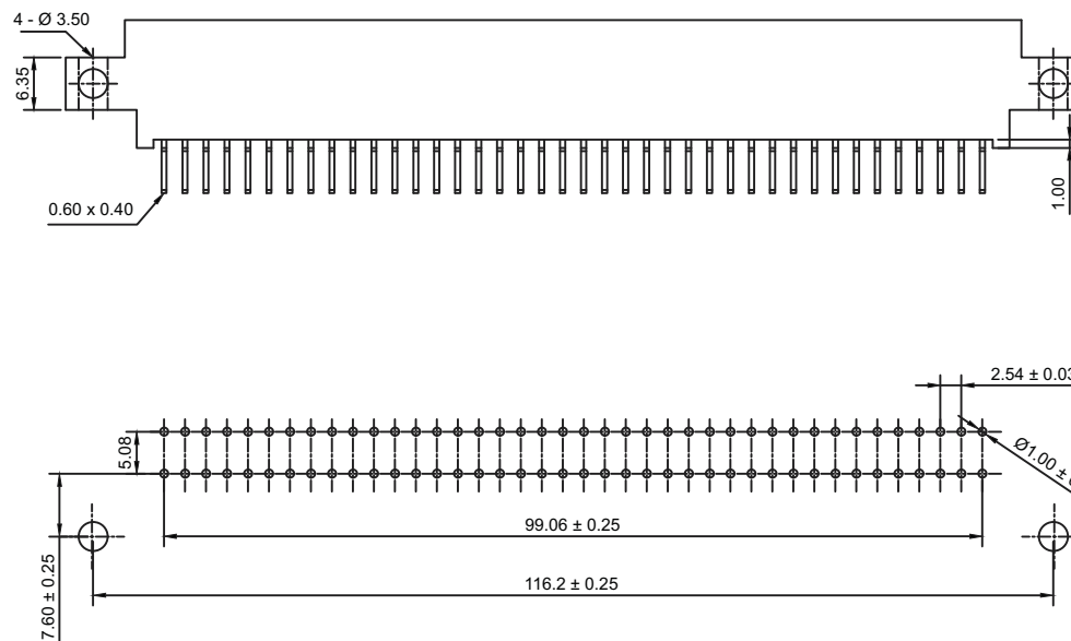
PCB Layout
