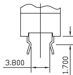
DETAIL OF KINKED
