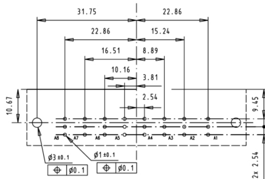
PCB layout, component side
